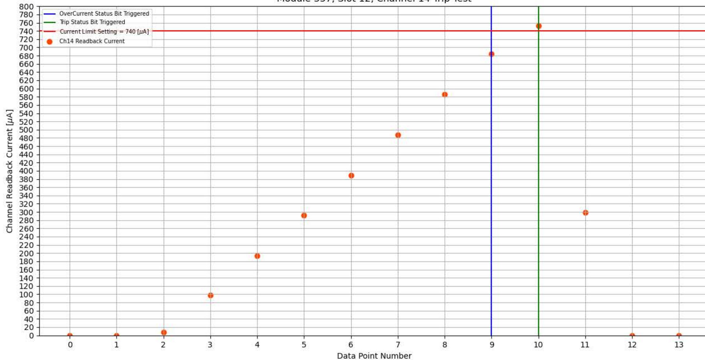
Module 337, Slot 12, Channel 14 Trip Test
