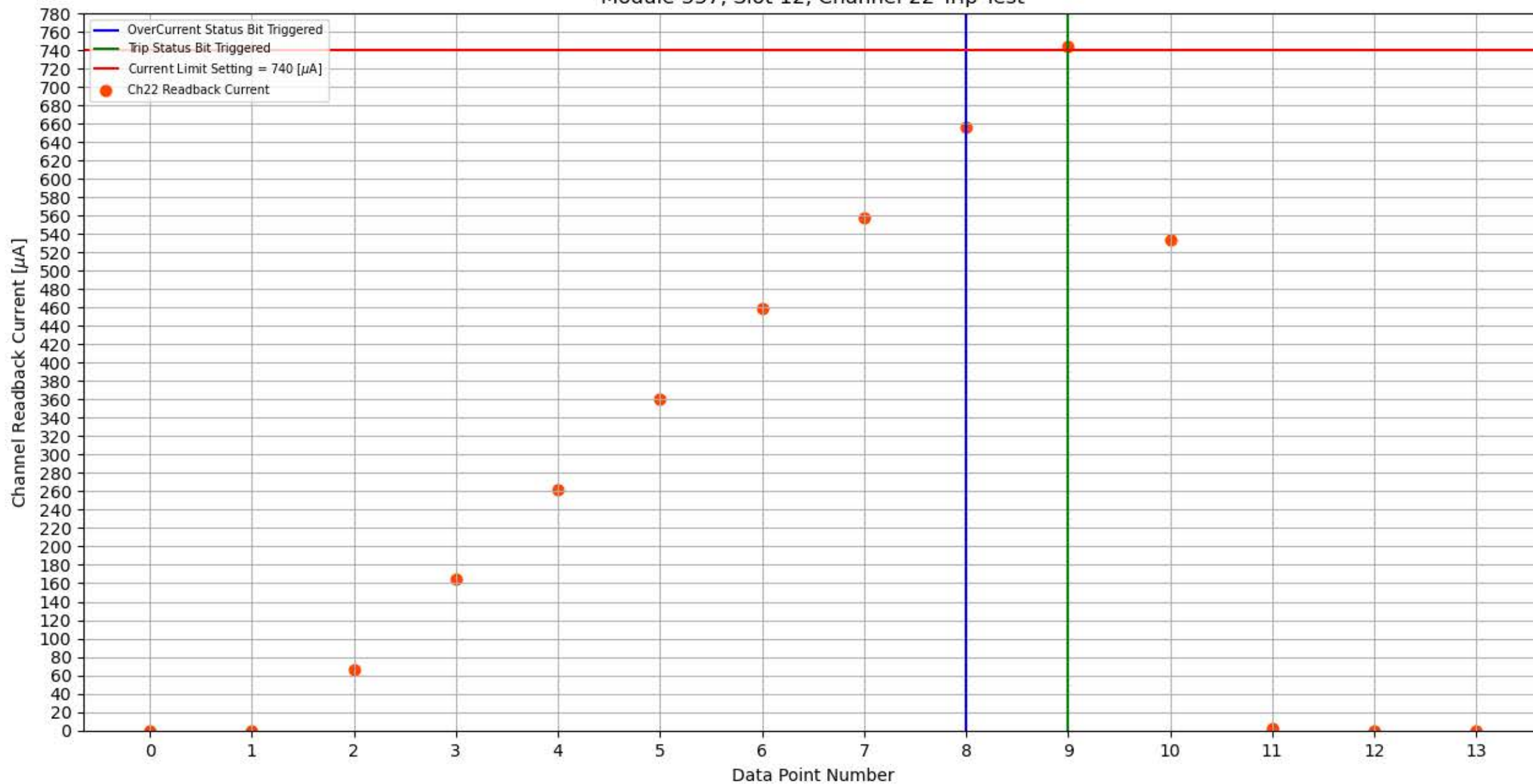
Module 337, Slot 12, Channel 22 Trip Test
