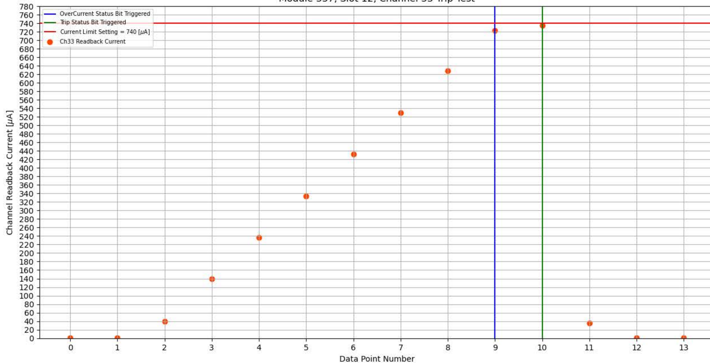
Module 337, Slot 12, Channel 33 Trip Test
