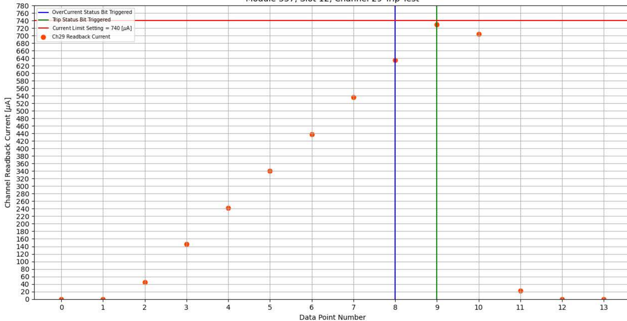
Module 337, Slot 12, Channel 29 Trip Test
