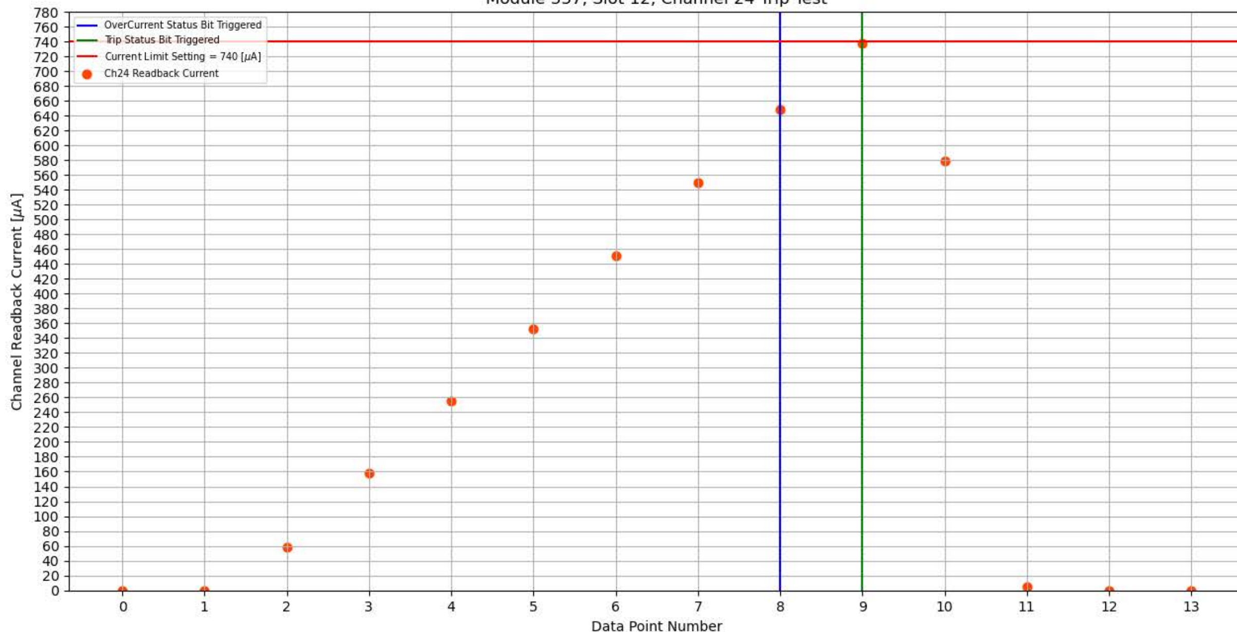
Module 337, Slot 12, Channel 24 Trip Test
