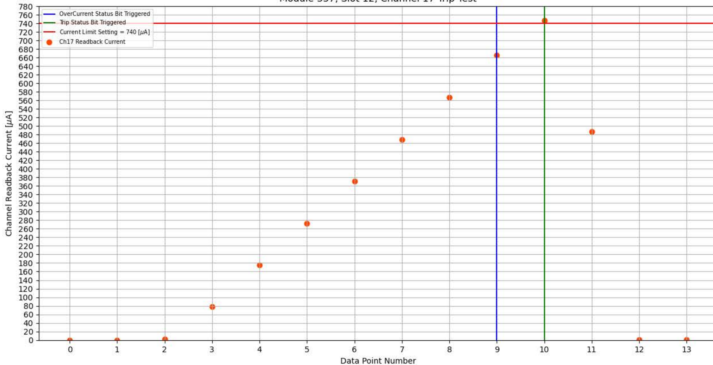
Module 337, Slot 12, Channel 17 Trip Test
