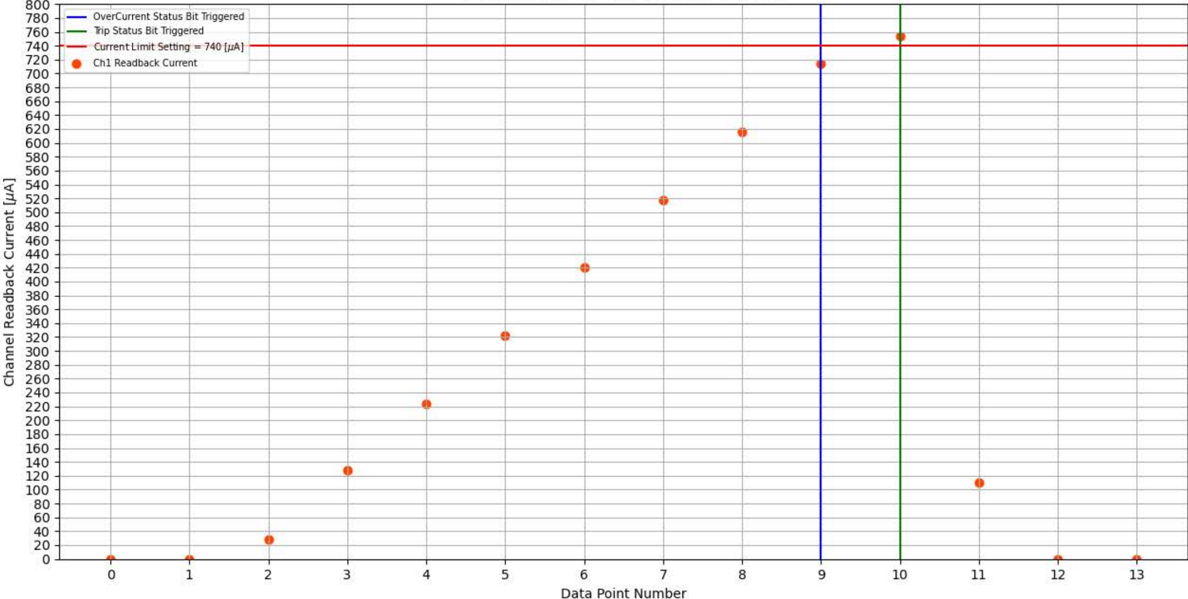
Module 337, Slot 12, Channel 1 Trip Test
