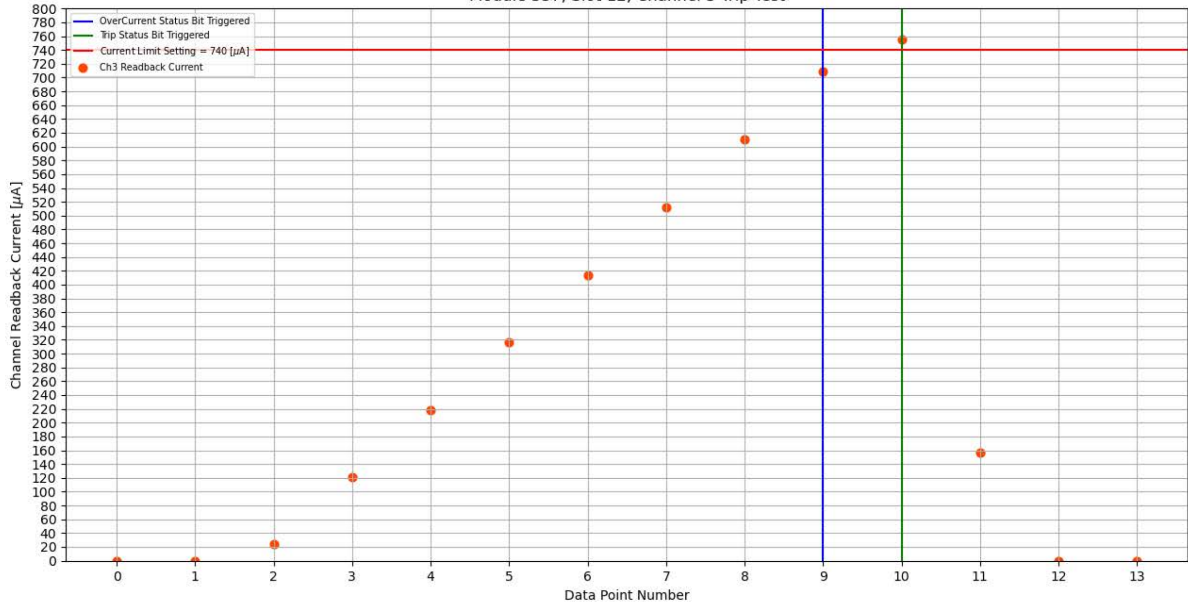
Module 337, Slot 12, Channel 3 Trip Test
