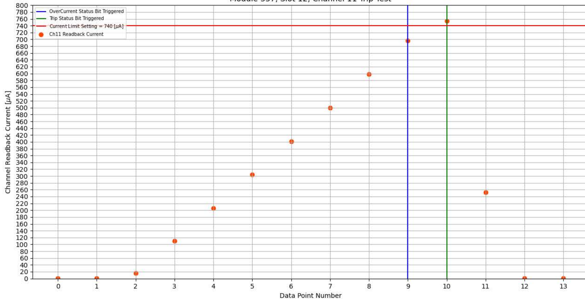
Module 337, Slot 12, Channel 11 Trip Test
