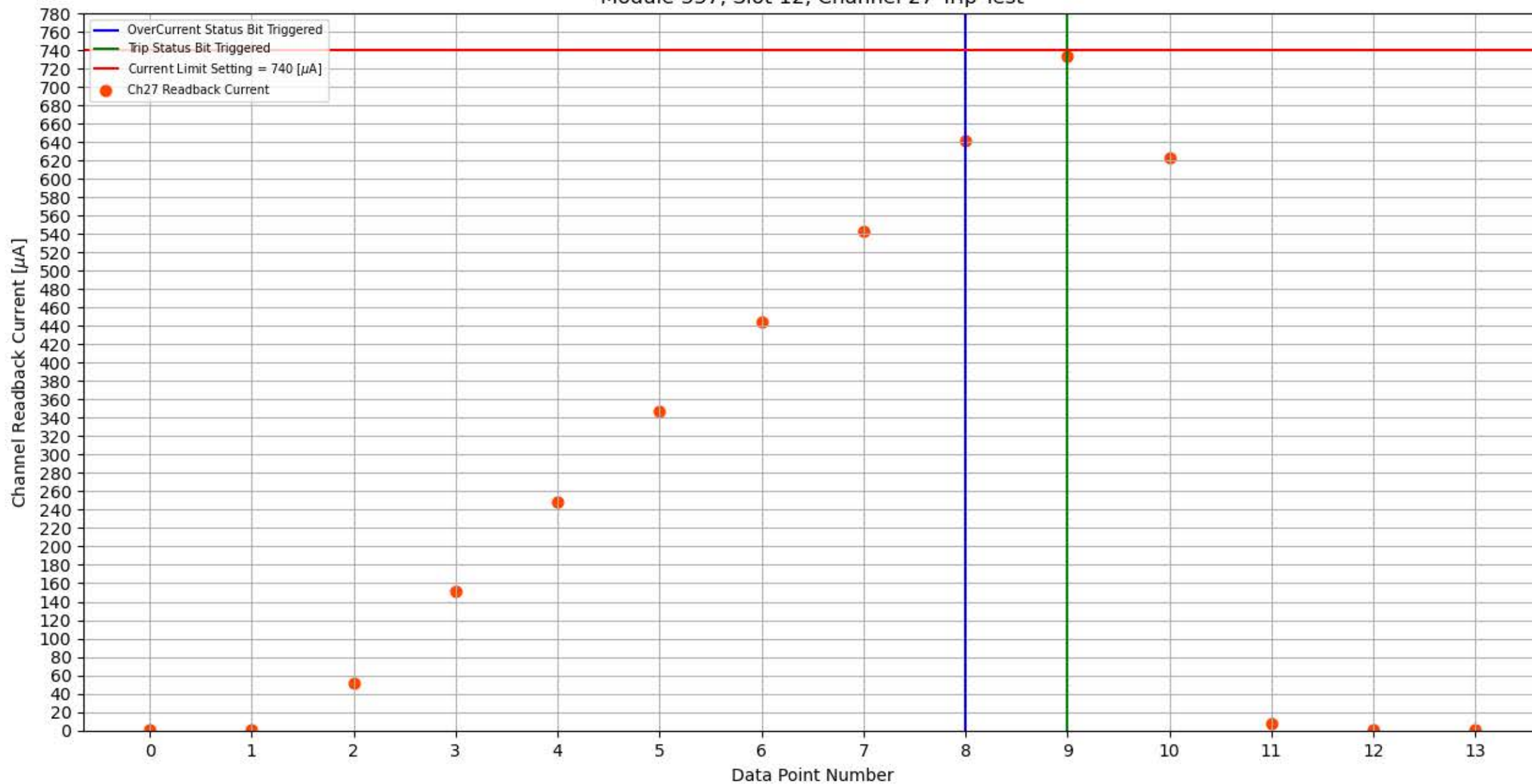
Module 337, Slot 12, Channel 27 Trip Test
