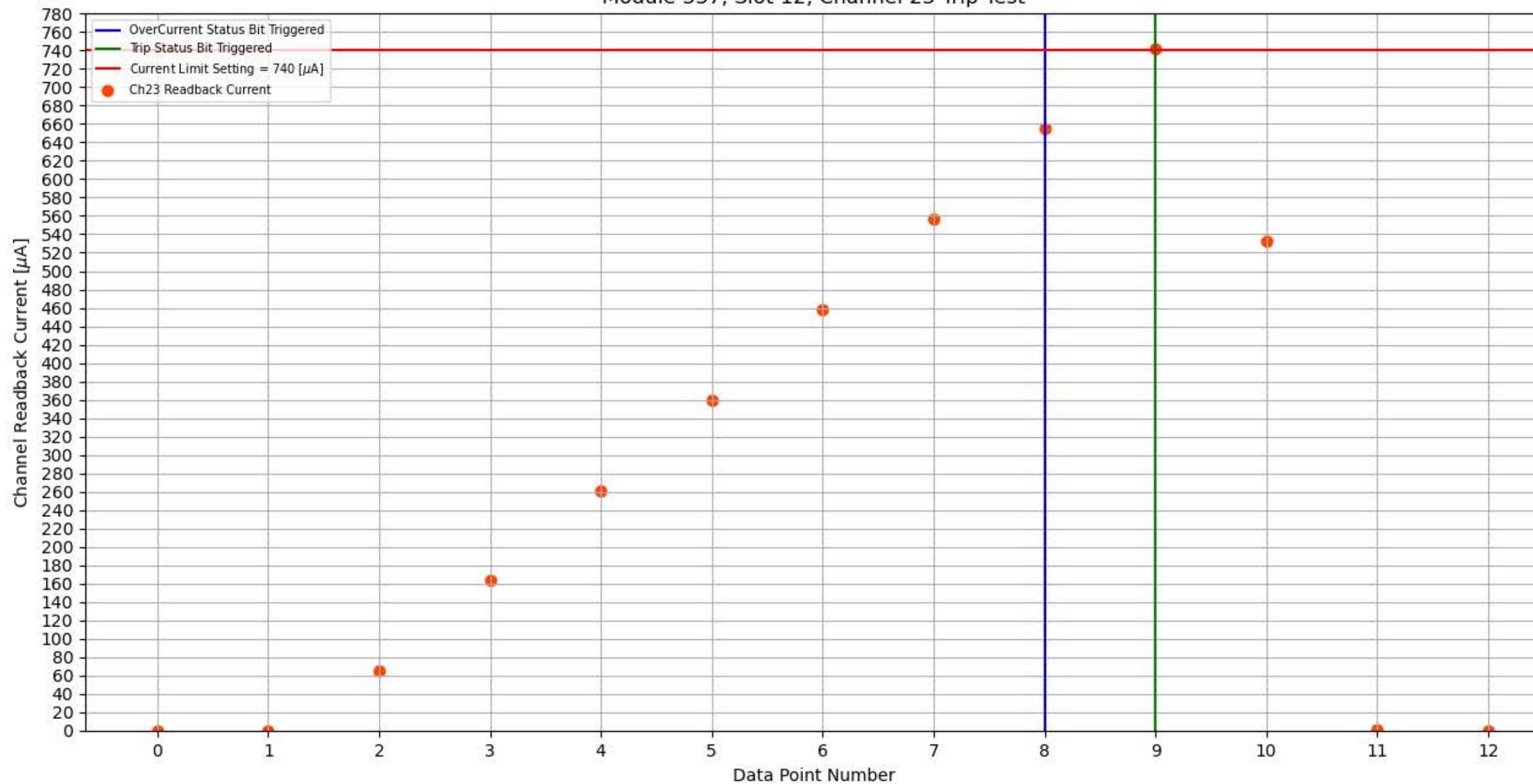
Module 337, Slot 12, Channel 23 Trip Test
