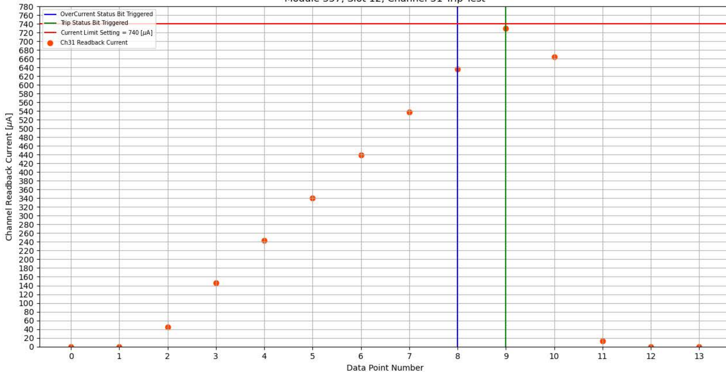
Module 337, Slot 12, Channel 31 Trip Test
