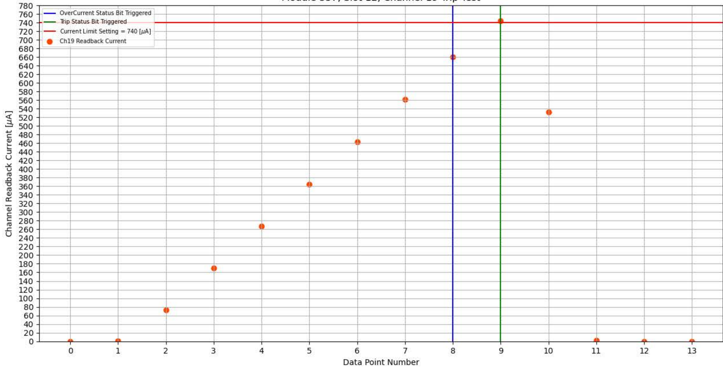
Module 337, Slot 12, Channel 19 Trip Test
