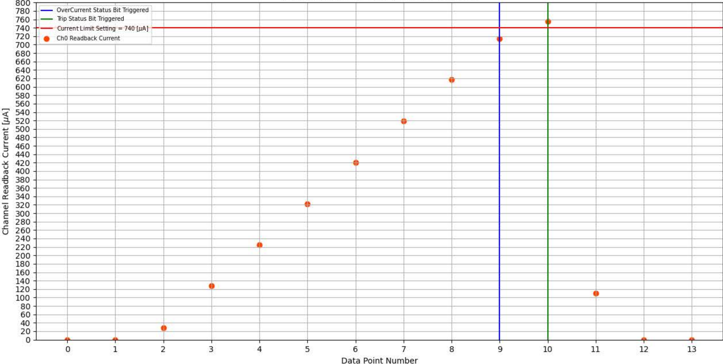
Module 337, Slot 12, Channel 0 Trip Test
