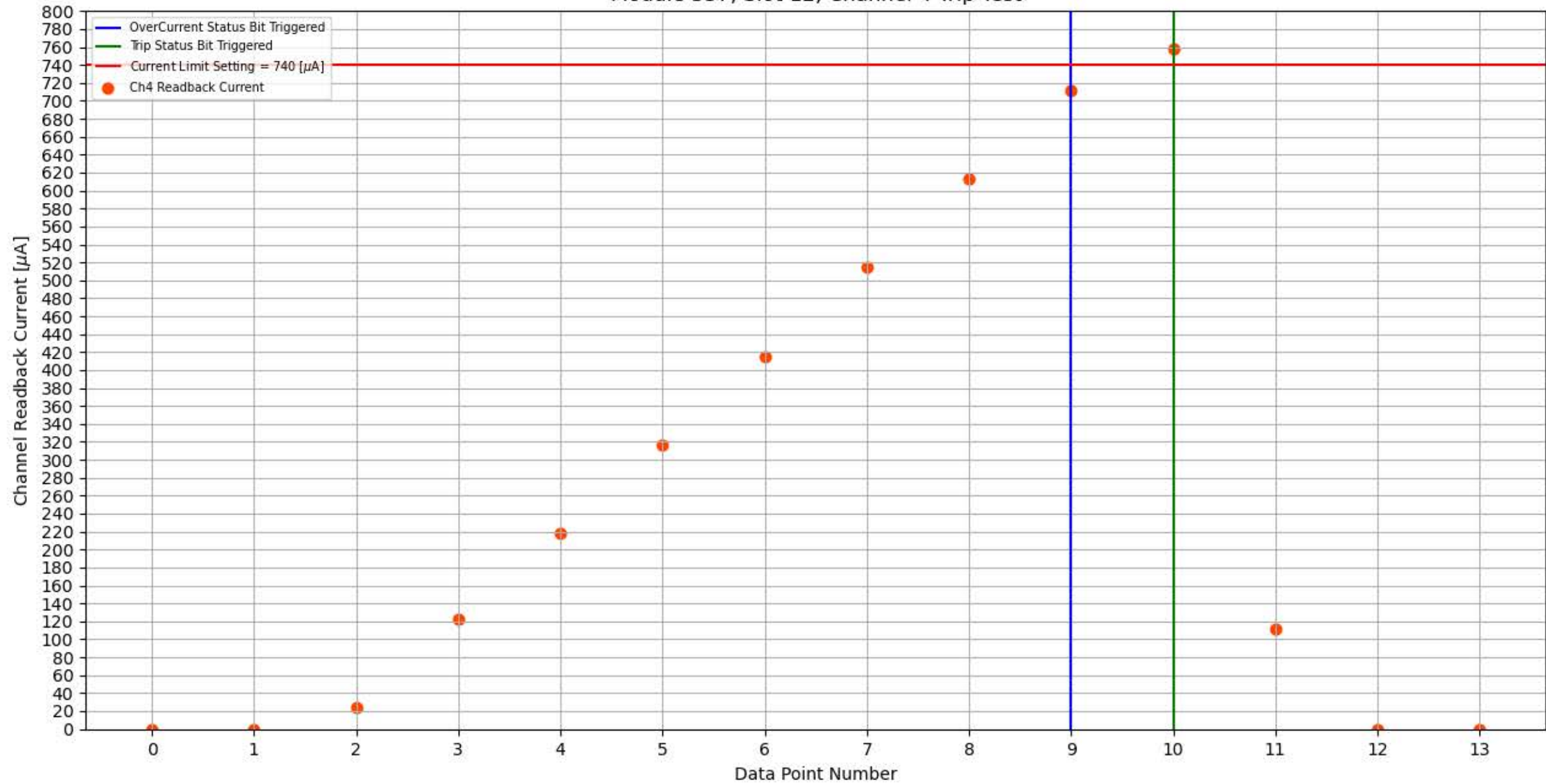
Module 337, Slot 12, Channel 4 Trip Test
