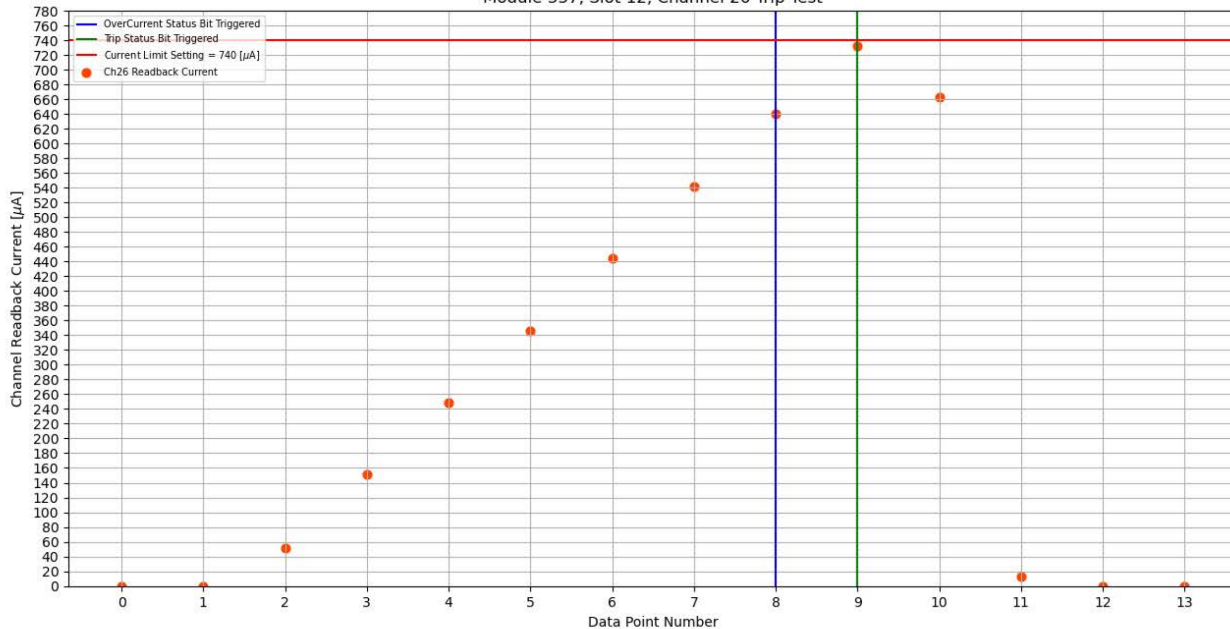
Module 337, Slot 12, Channel 26 Trip Test
