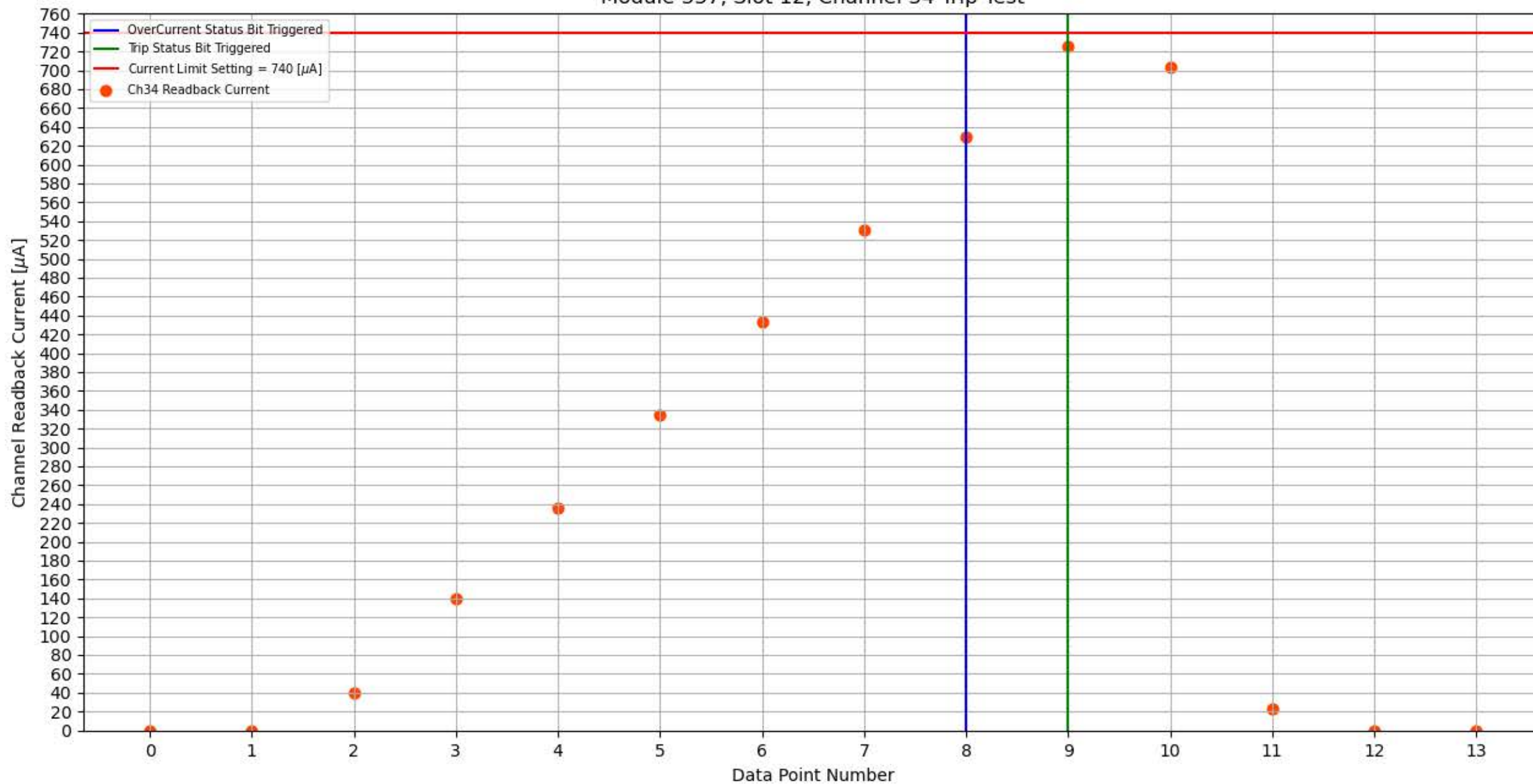
Module 337, Slot 12, Channel 34 Trip Test
