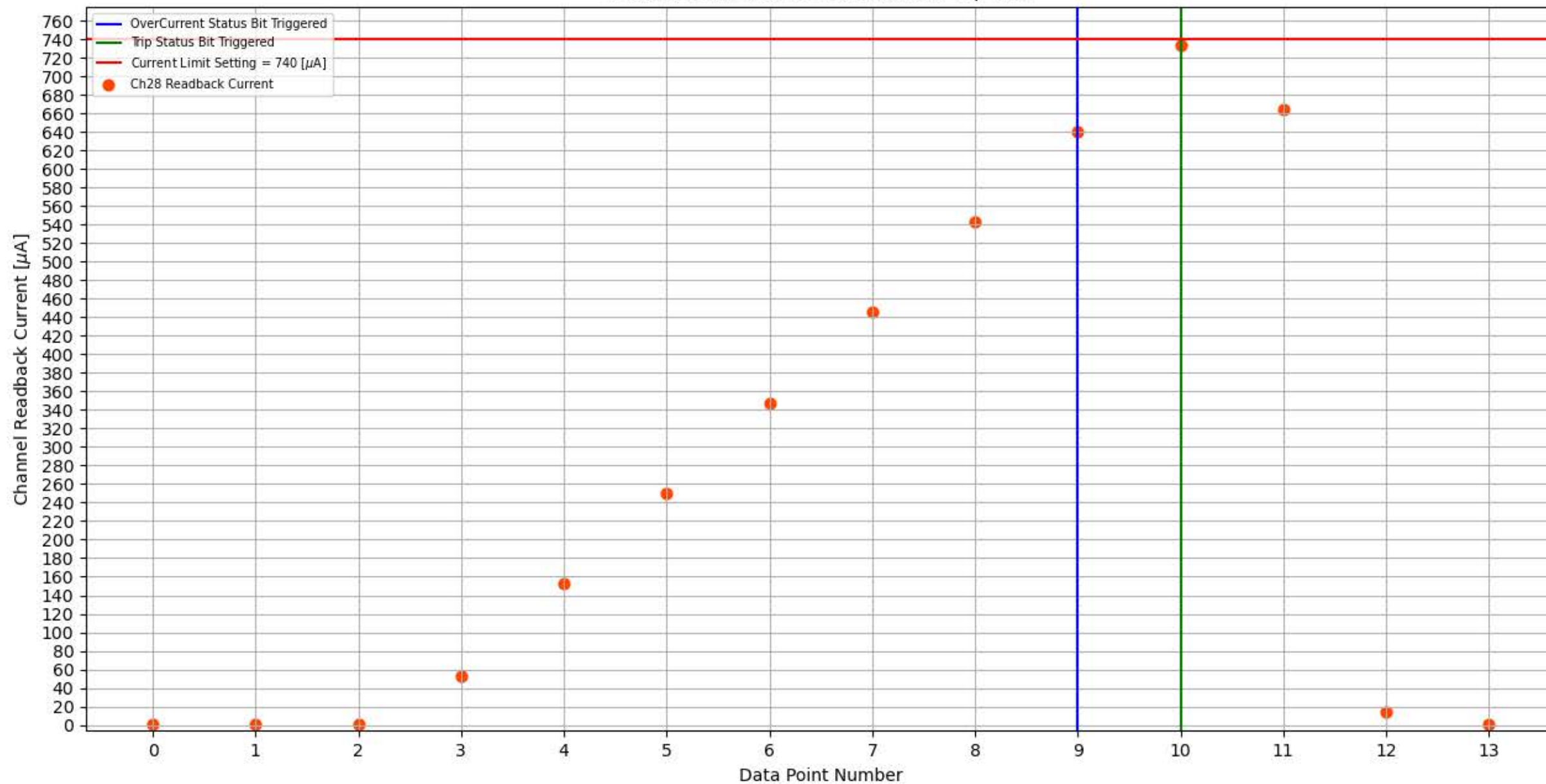
Module 337, Slot 12, Channel 28 Trip Test
