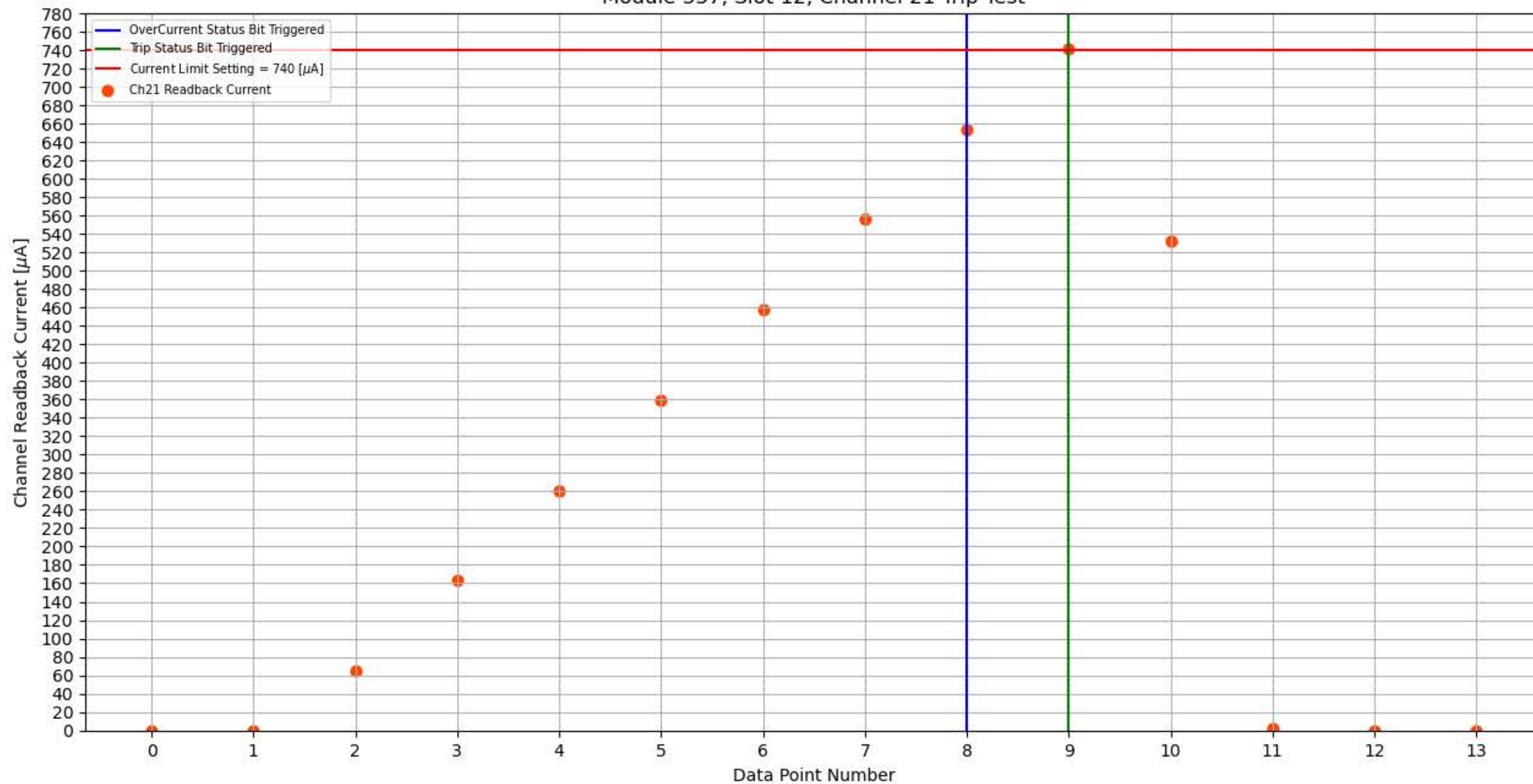
Module 337, Slot 12, Channel 21 Trip Test
