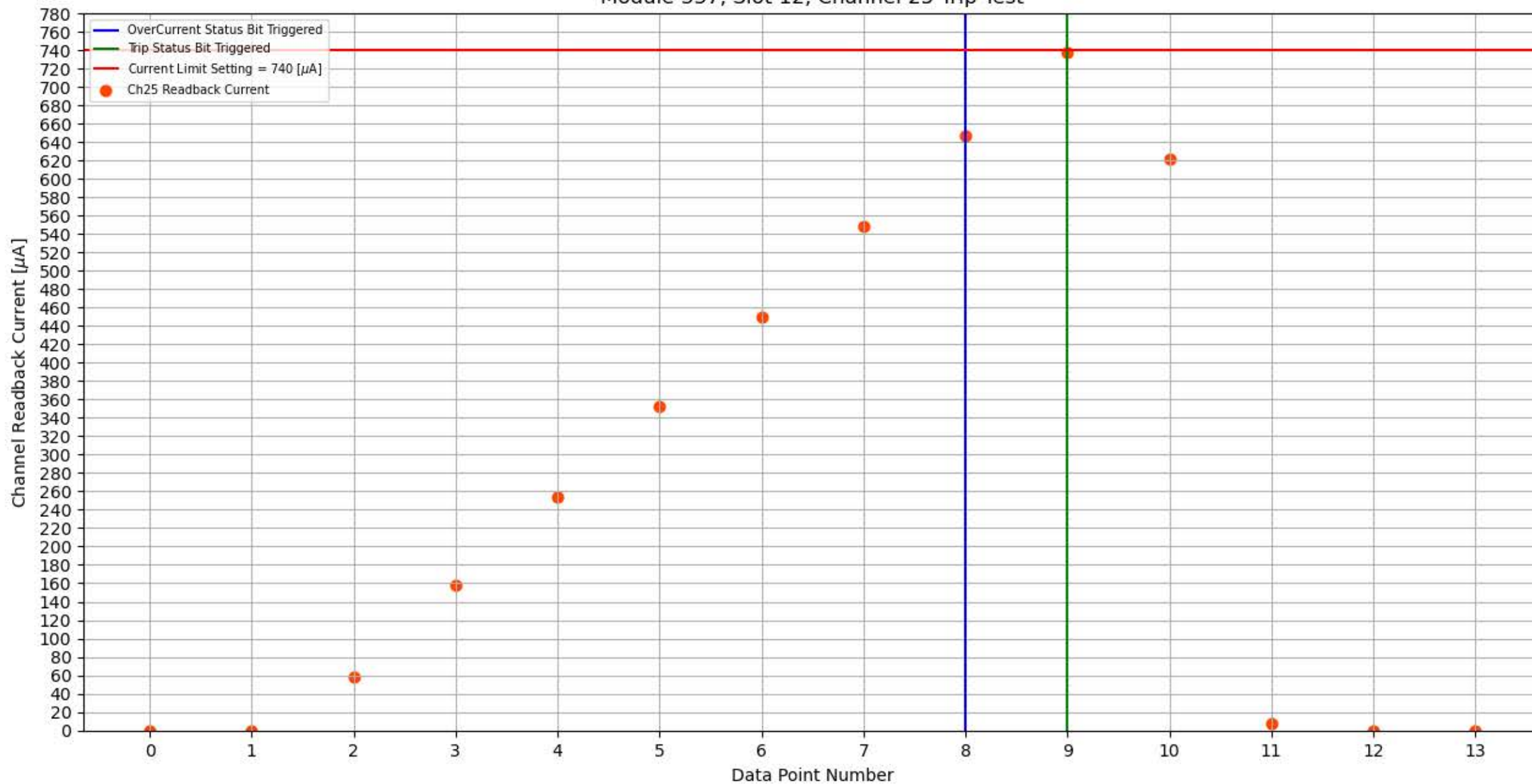
Module 337, Slot 12, Channel 25 Trip Test
