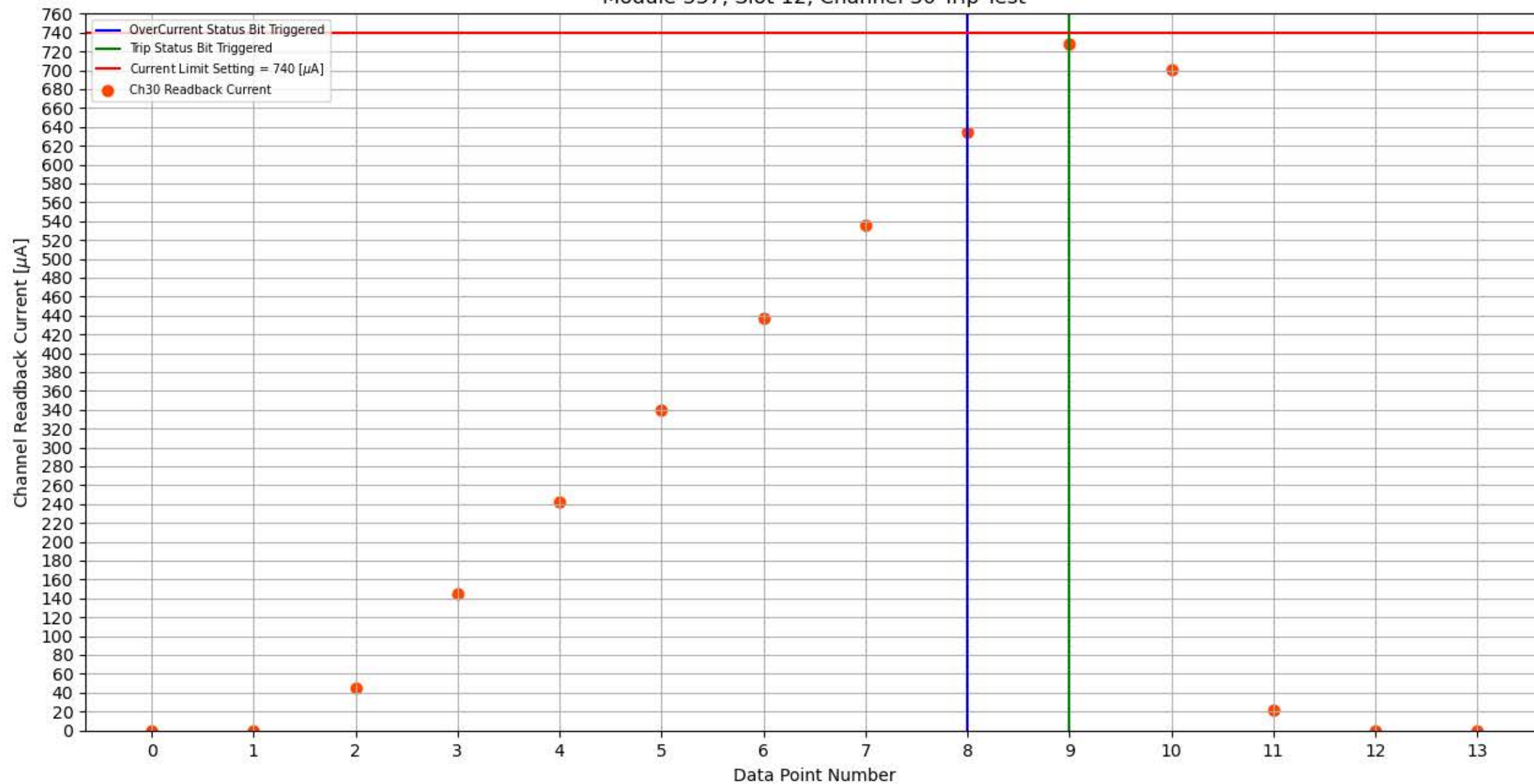
Module 337, Slot 12, Channel 30 Trip Test
