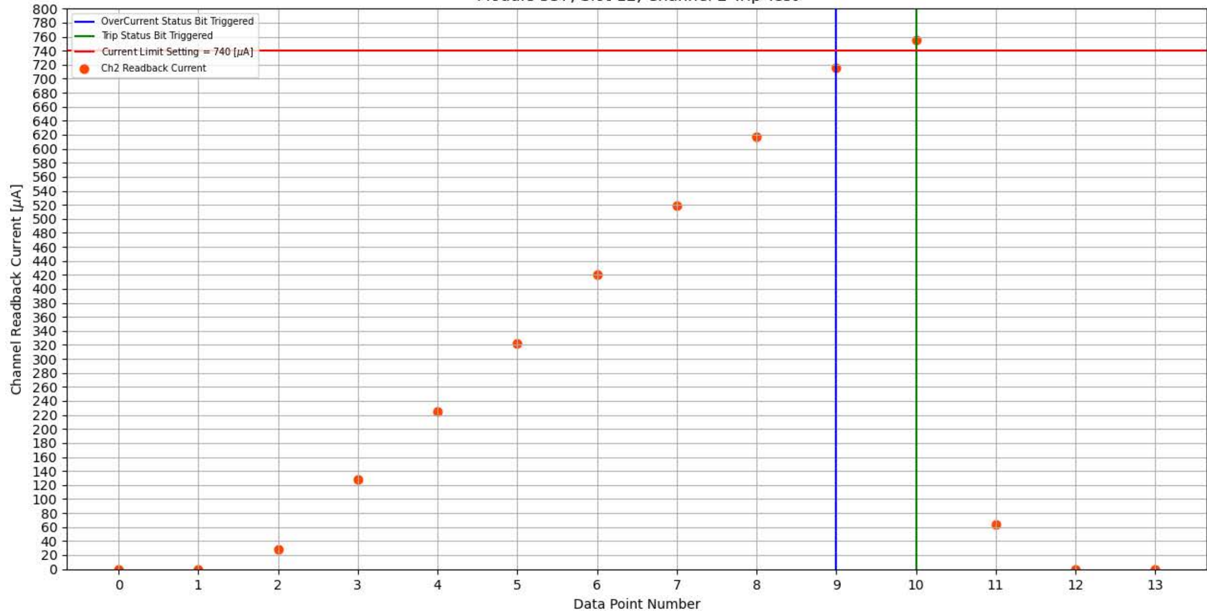
Module 337, Slot 12, Channel 2 Trip Test
