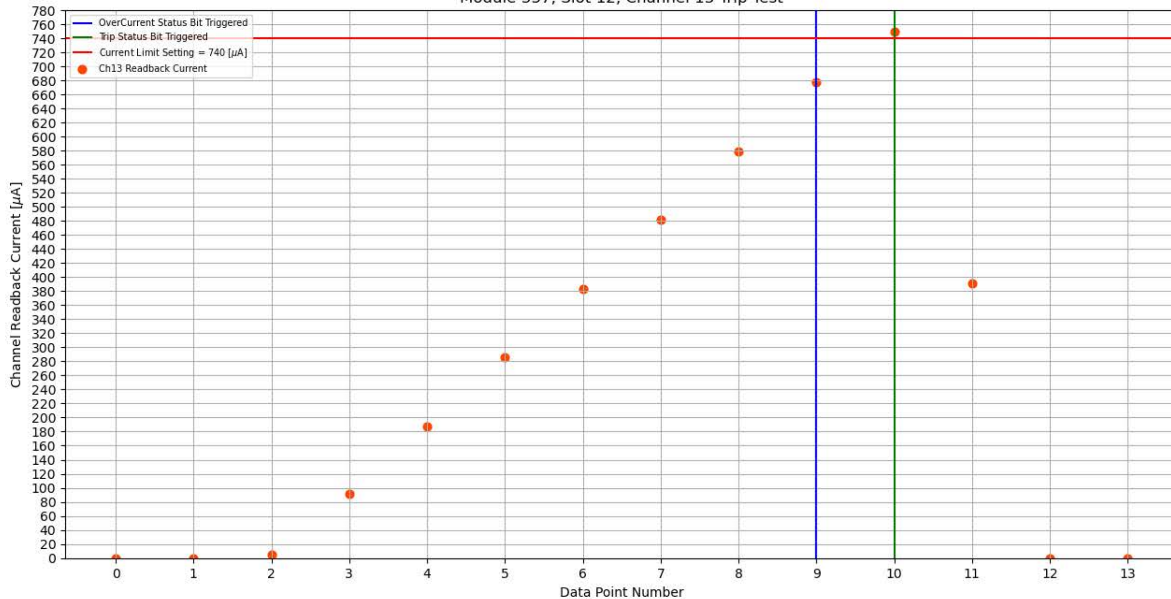
Module 337, Slot 12, Channel 13 Trip Test
