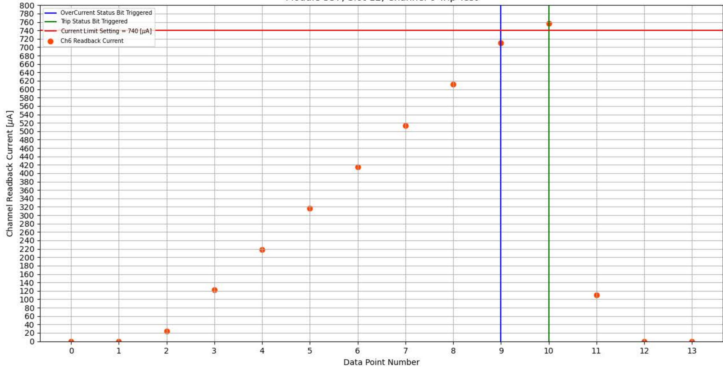
Module 337, Slot 12, Channel 6 Trip Test
