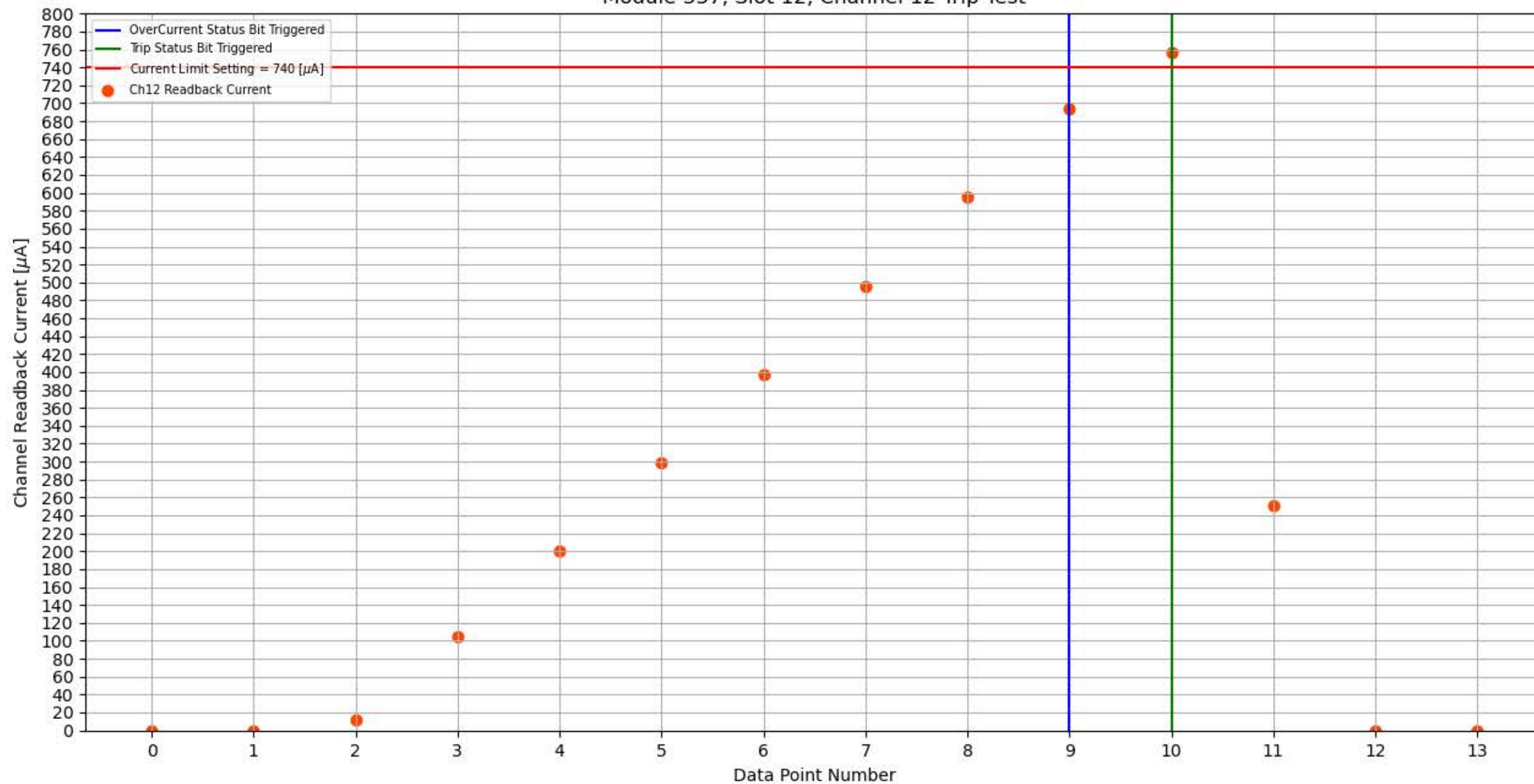
Module 337, Slot 12, Channel 12 Trip Test
