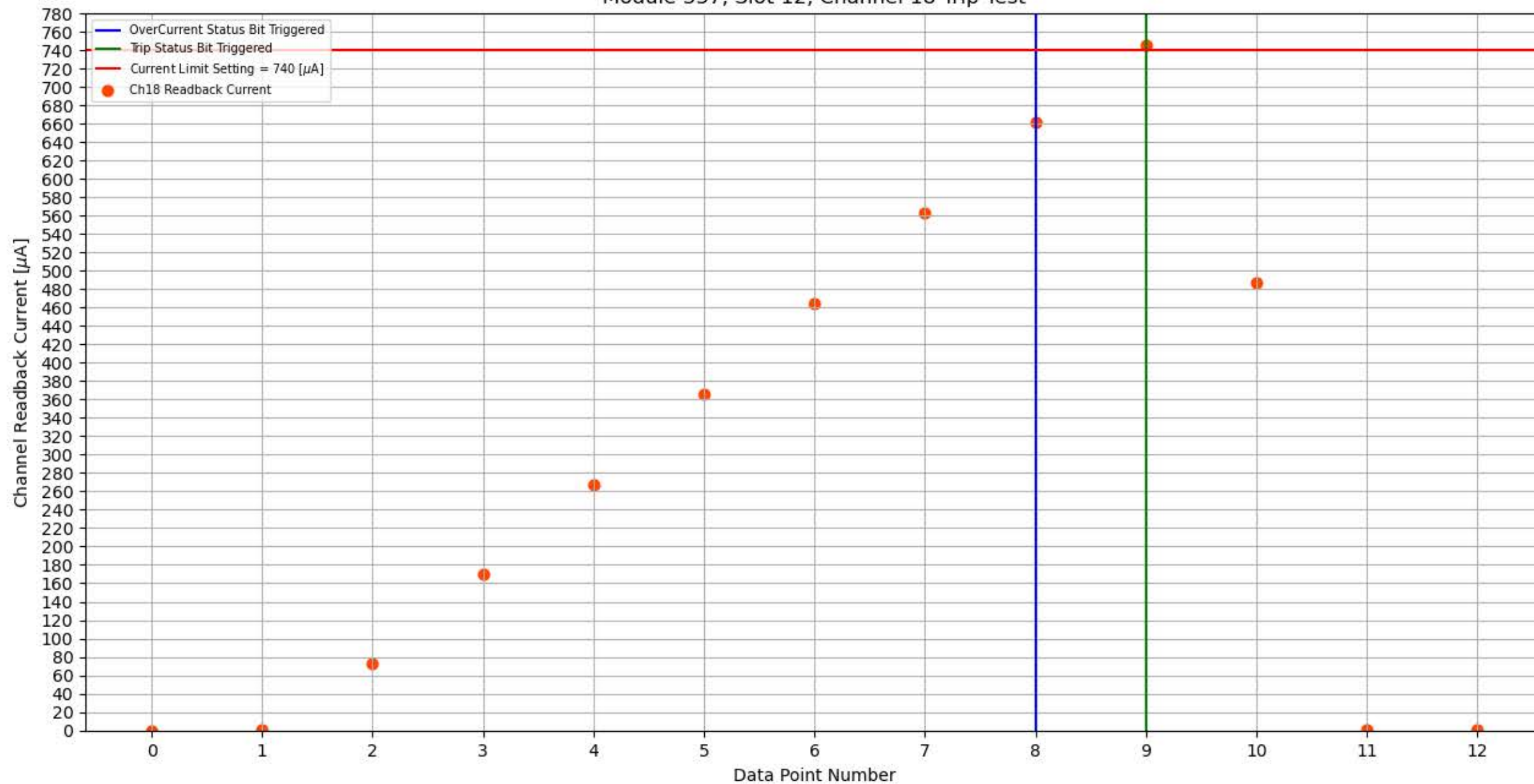
Module 337, Slot 12, Channel 18 Trip Test
