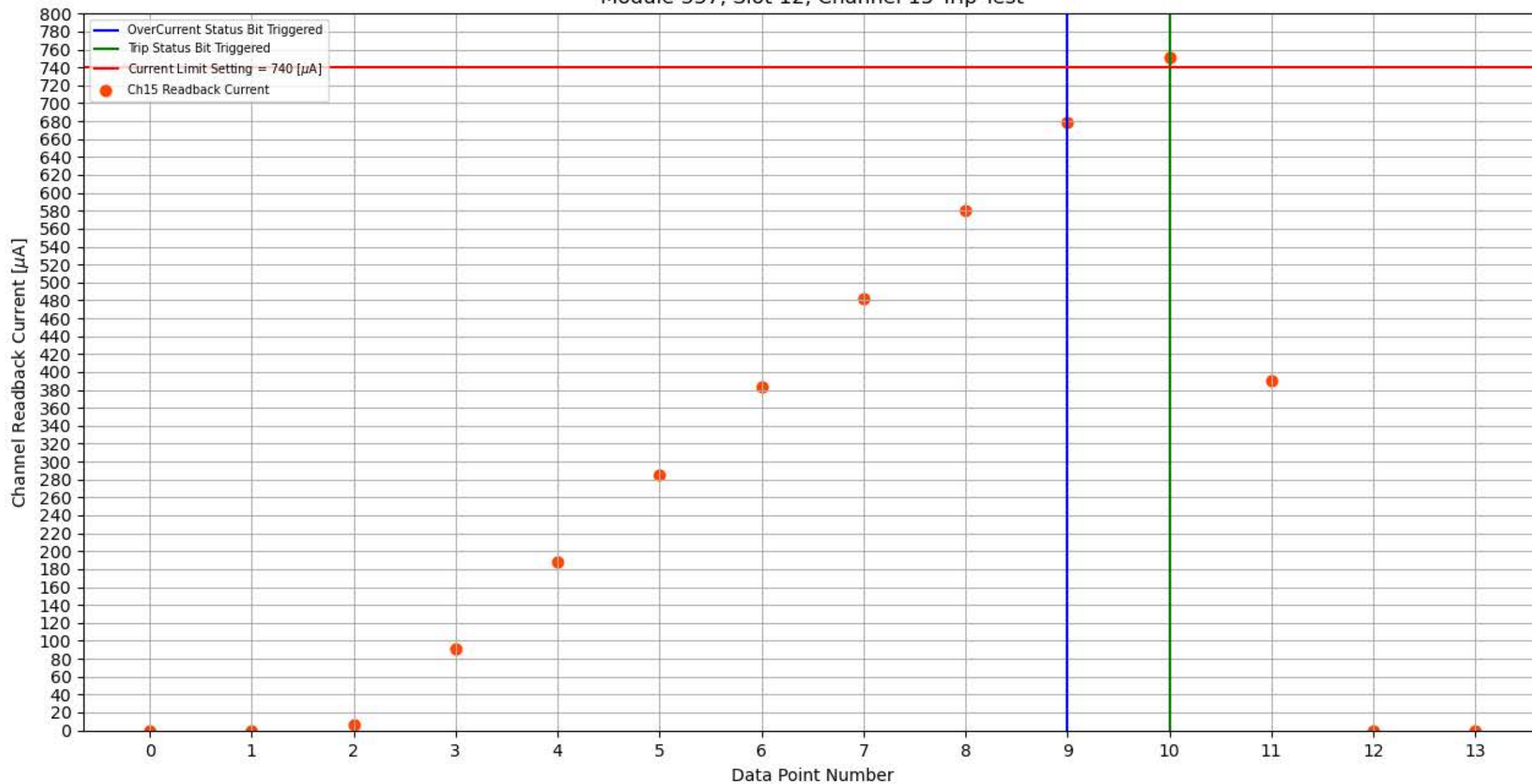
Module 337, Slot 12, Channel 15 Trip Test
