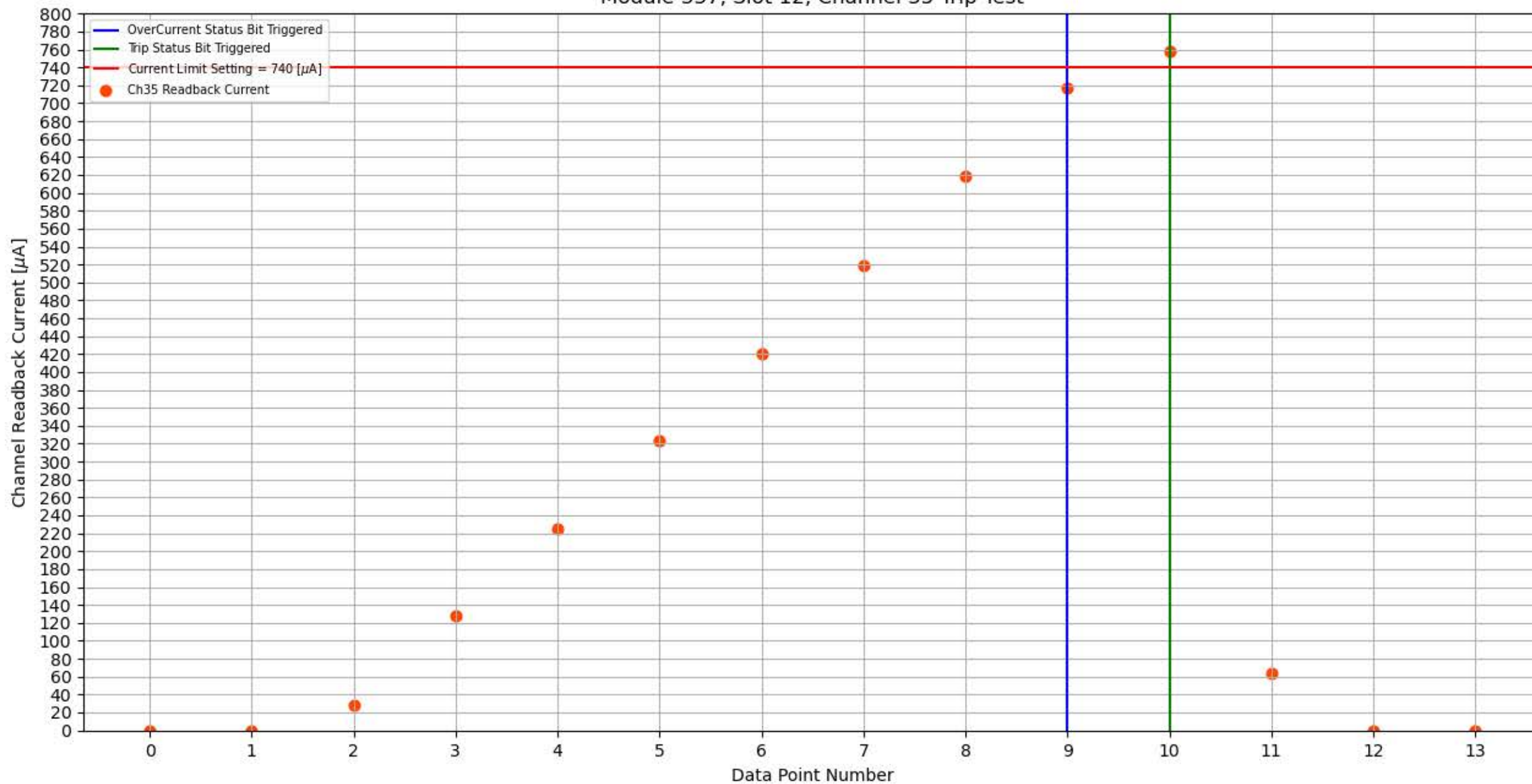
Module 337, Slot 12, Channel 35 Trip Test
