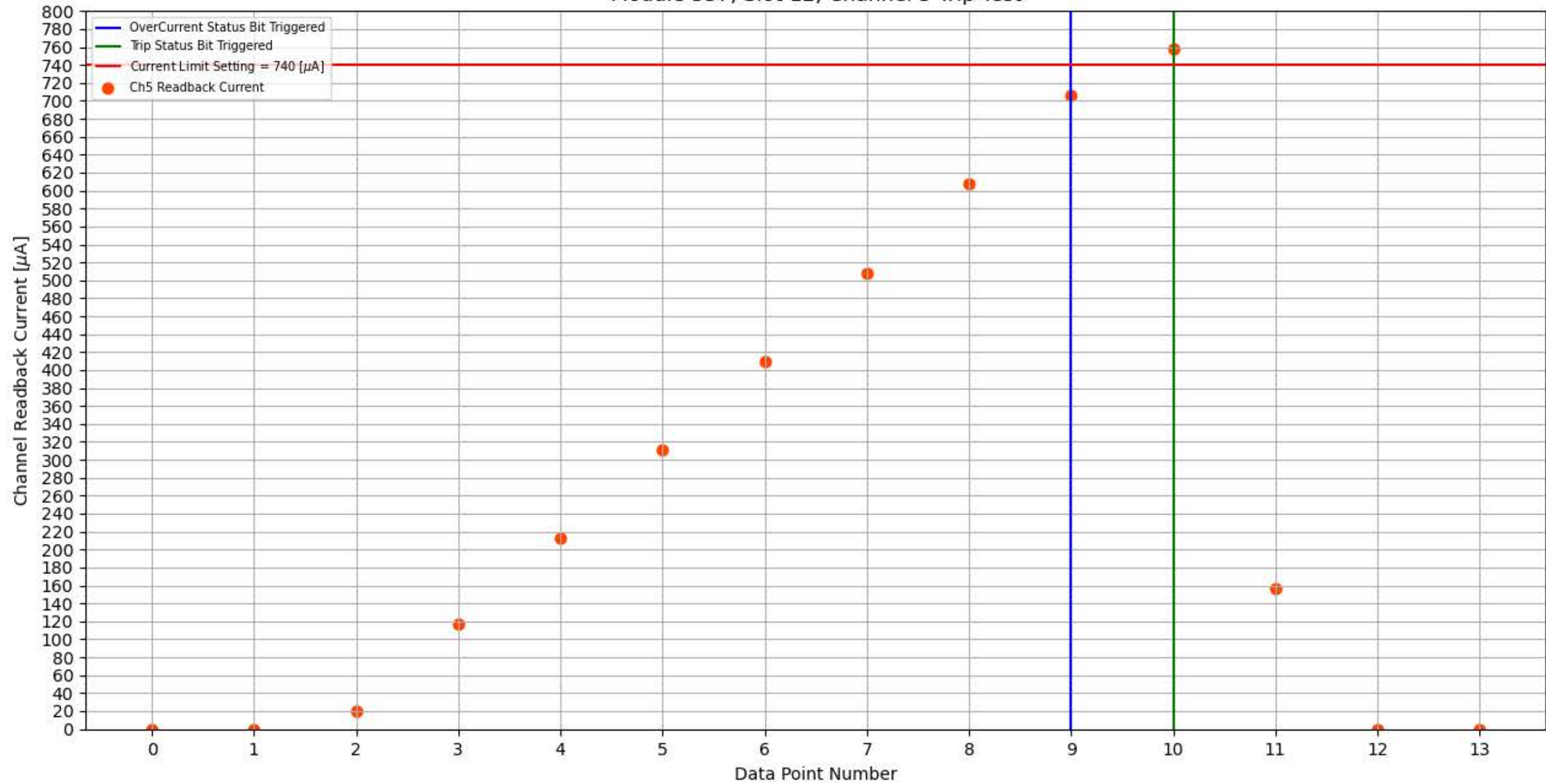
Module 337, Slot 12, Channel 5 Trip Test
