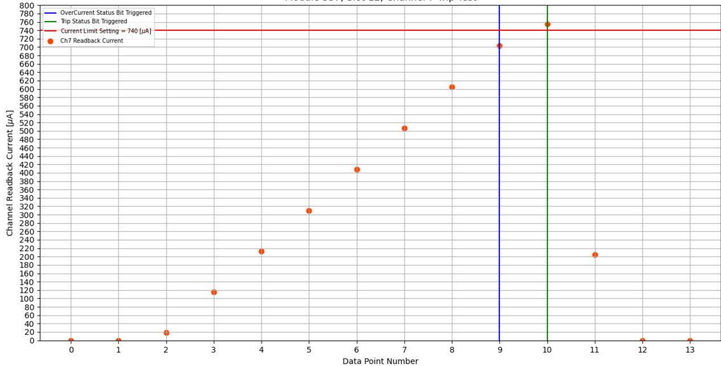
Module 337, Slot 12, Channel 7 Trip Test
