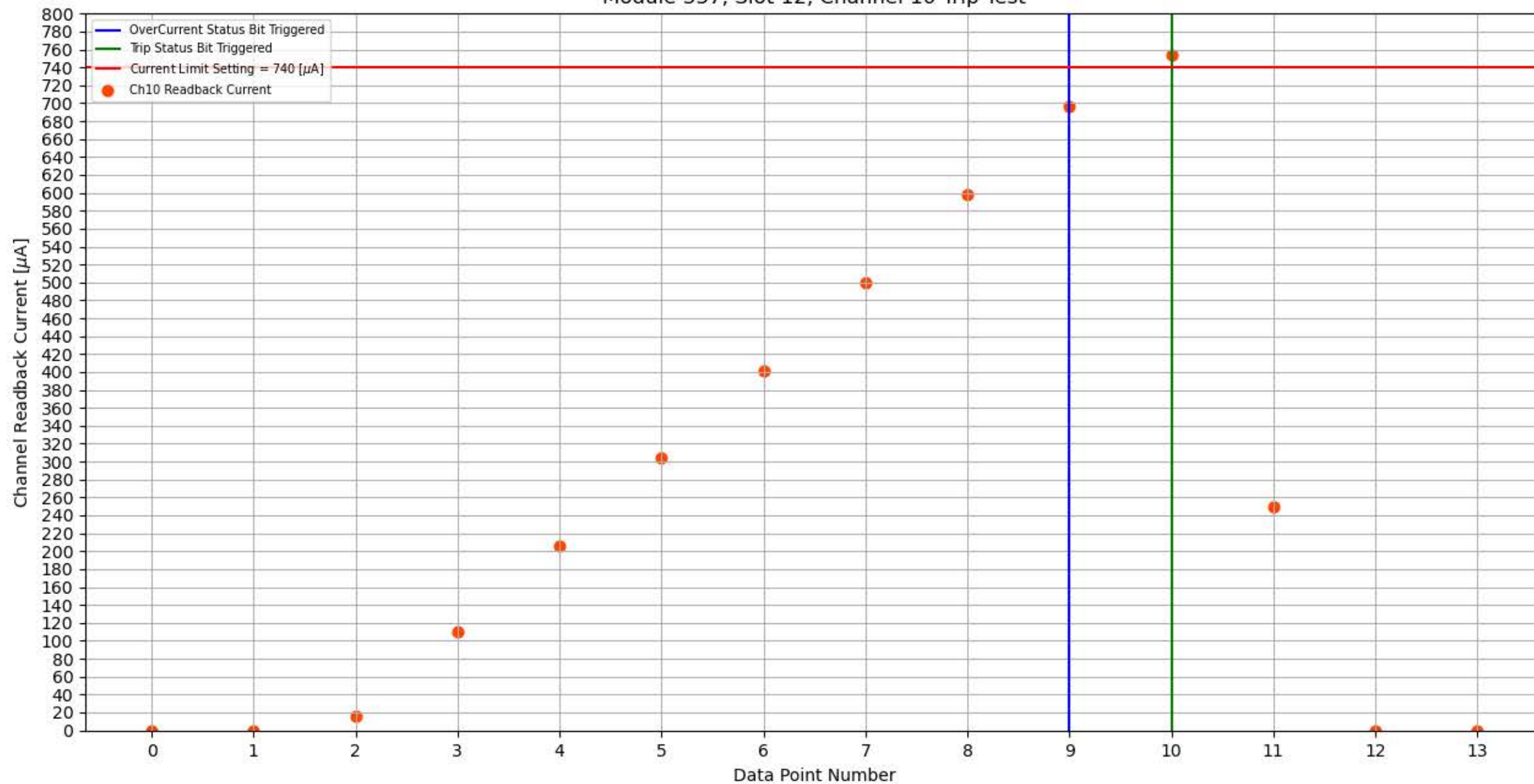
Module 337, Slot 12, Channel 10 Trip Test
