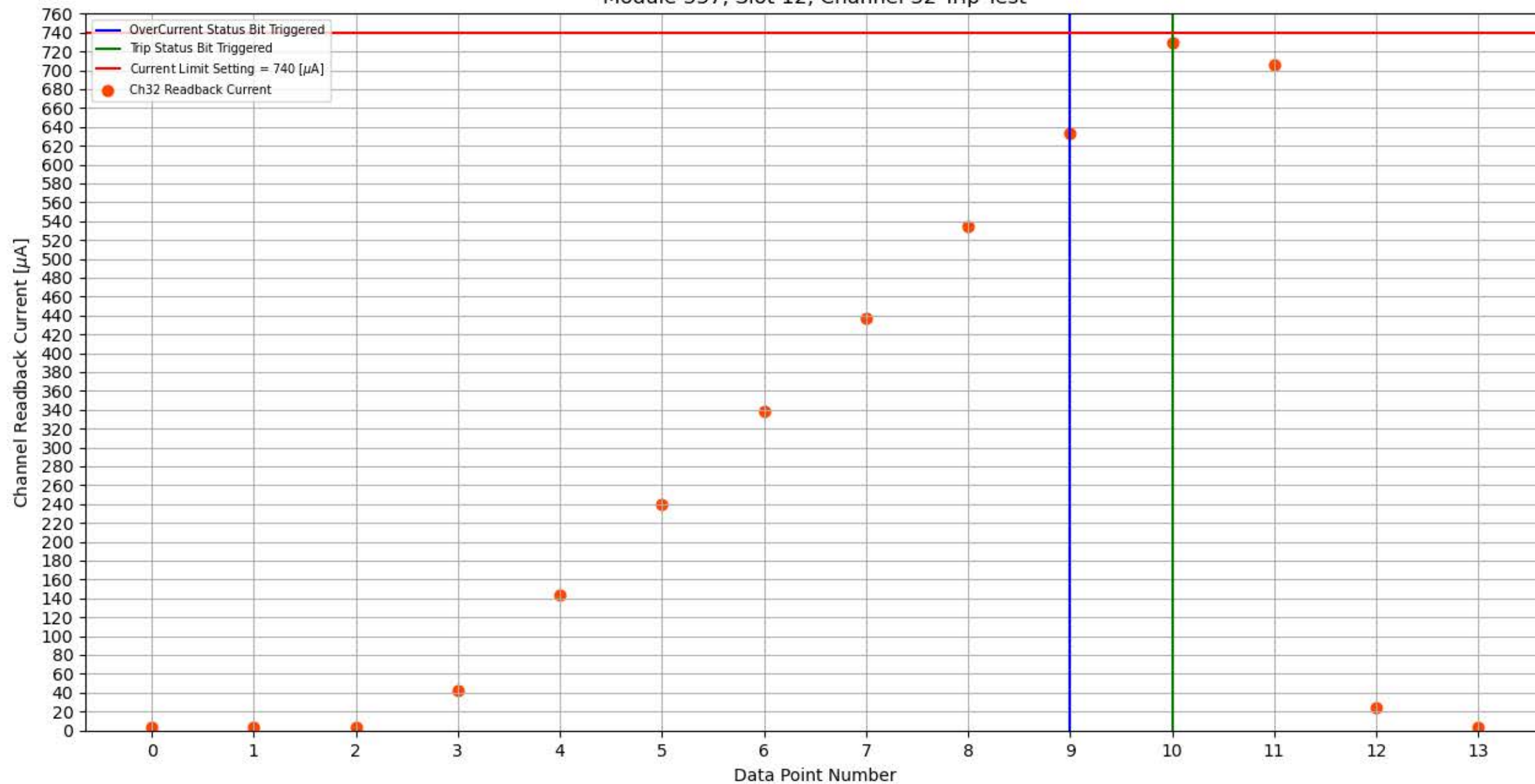
Module 337, Slot 12, Channel 32 Trip Test
