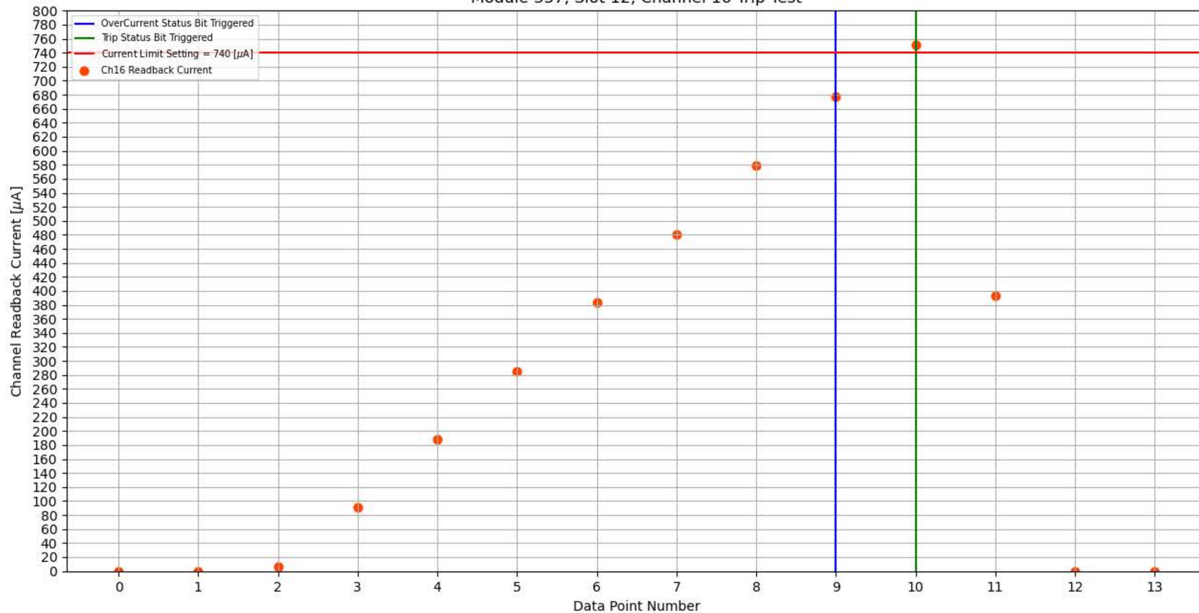
Module 337, Slot 12, Channel 16 Trip Test
