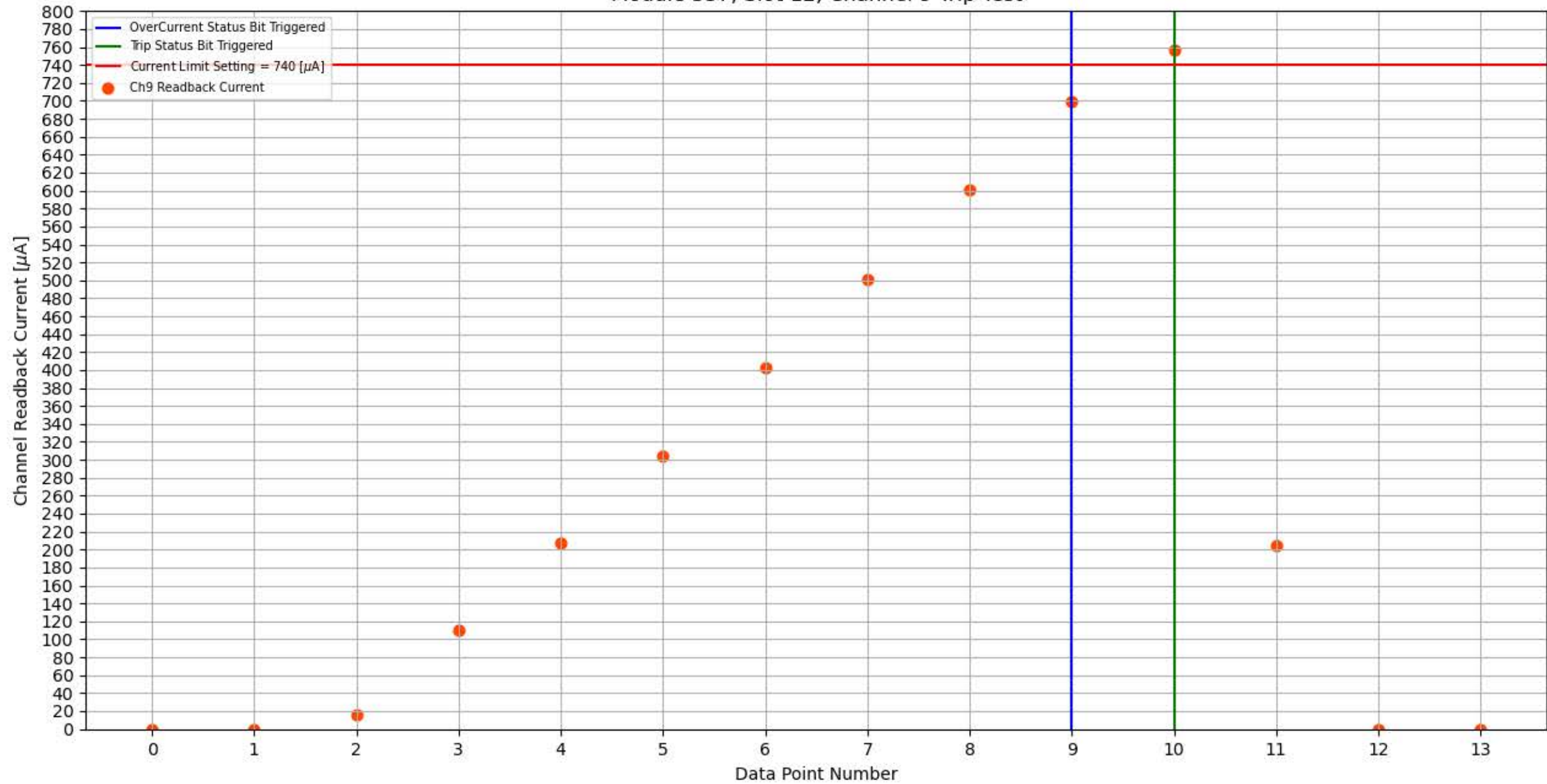
Module 337, Slot 12, Channel 9 Trip Test
