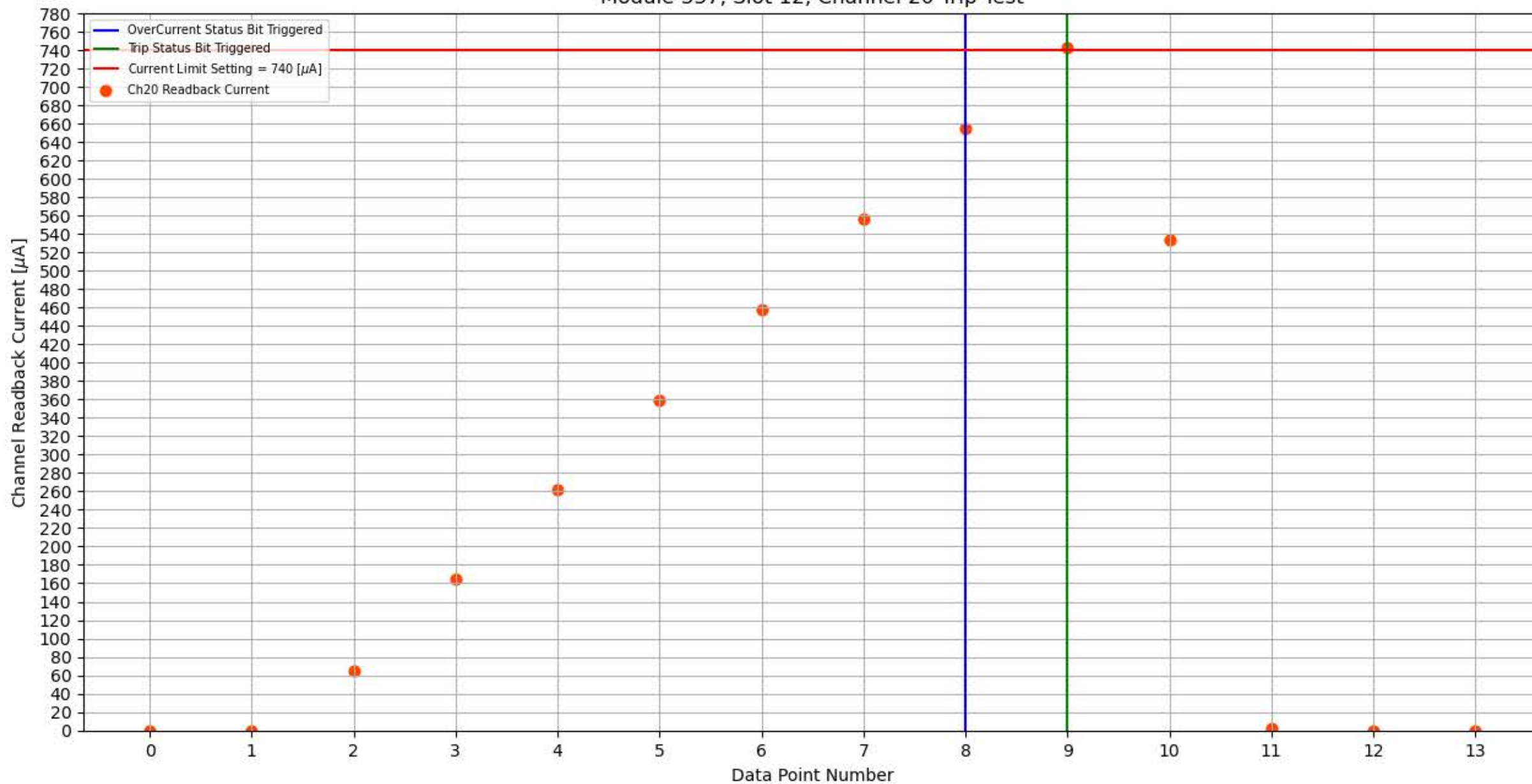
Module 337, Slot 12, Channel 20 Trip Test
