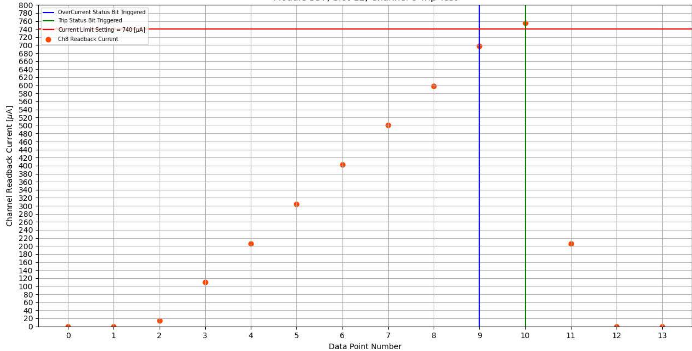
Module 337, Slot 12, Channel 8 Trip Test
